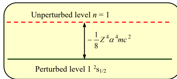
Figure 9. Effect of the fine-structure Hamiltonian on the ground state 1^2s_{1/2} of the hydrogen-like systems.
