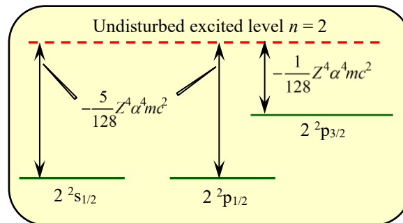
Figure 10. Effect of the fine-structure Hamiltonian on the first excited state n = 2 of the hydrogen-like systems. The splitting of the 2^2p_{1/2} and 2^2s_{1/2} states is not resolved with the framework of the Dirac's model.
