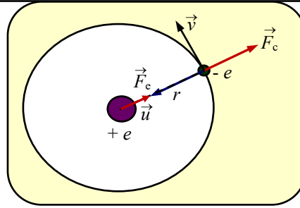
Figure 4. Forces applied to the electron of the hydrogen atom.
