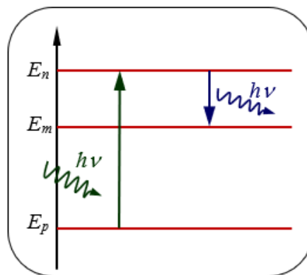
Figure 1. Electronic transitions.
