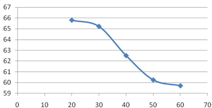
Figure 10. Percentage Change in COD Values with Variations in Congo Red Concentration
