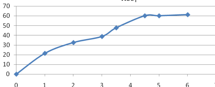
Figure 2. Graph of Percentage Change in Absorbance of TiO2 Catalyst Amount
