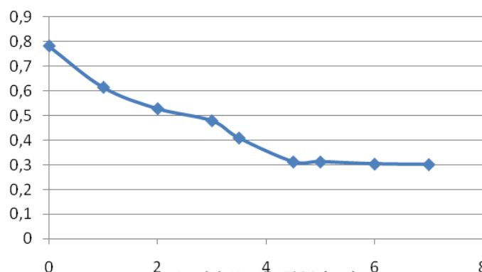
Figure 1. Graph of Changes in Absorbance Intensity of Congo Red Solution Against the Amount of TiO2 Catalyst
