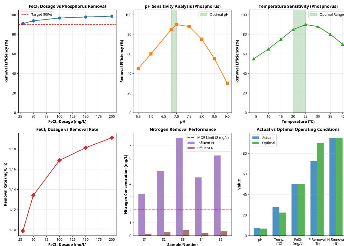
Figure 3. \text{FeCl}_3 Dosage vs. Phosphorus Removal Efficiency and Sensitivity Analysis
