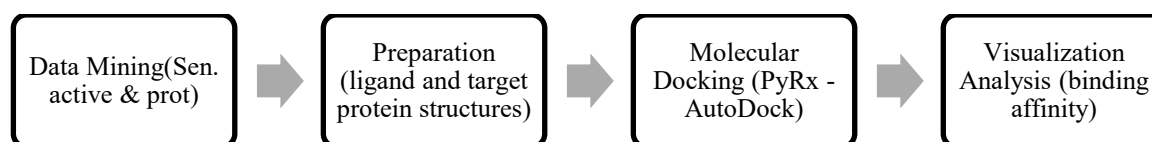
Figure 1. Flowchart of Research Procedure
