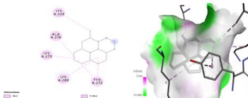
Figure 4. Interaction of Hexadecahydro-pyrene with PBP2a
