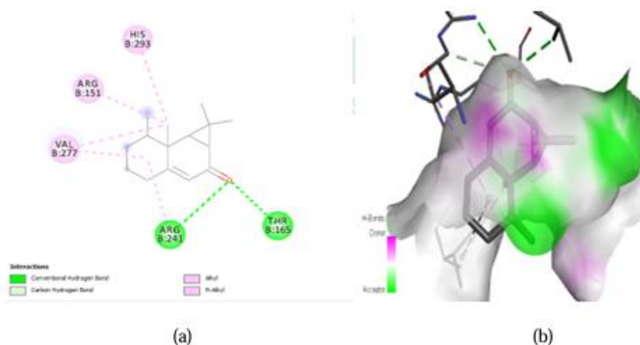
Figure 3. Interaction of Aristolone with mutant penicillin-binding protein 2a (PBP2a or PBP2').
