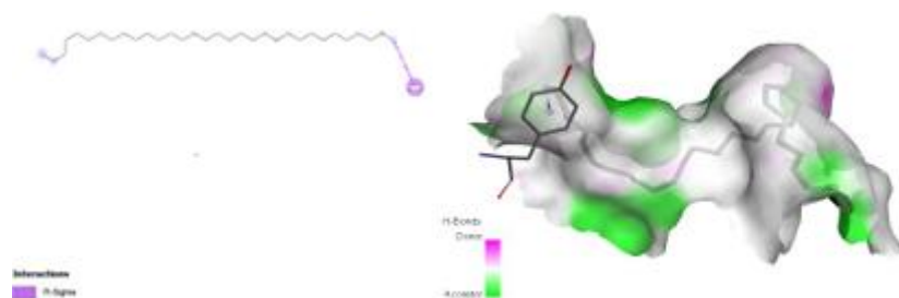
Figure 5. Interaction of Dotriacontane with PBP2a
