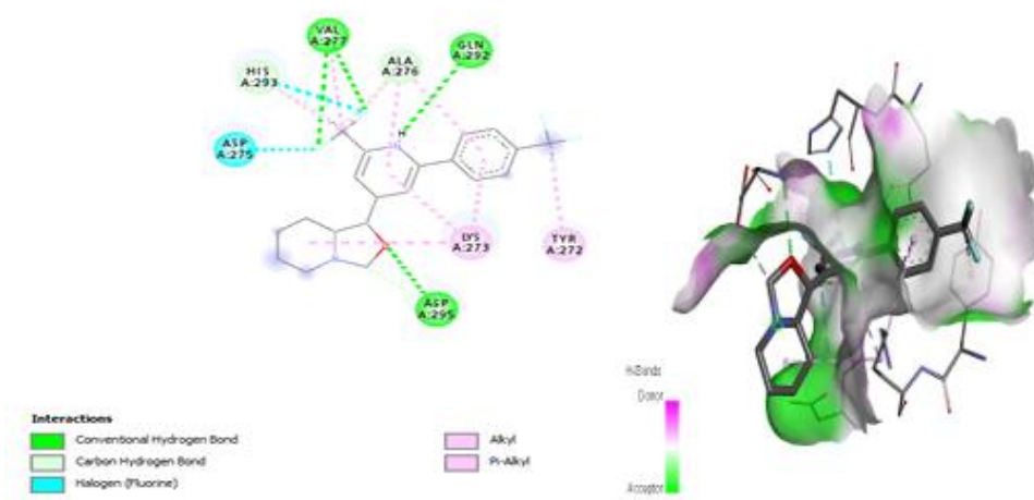
Figure 2. Interaction of Hexahydro-3H-cyclopenta[a]pentalen-3-one, 2,4a,5,6,7,8-hexahydro-4,4,7a-trimethyl-, (4aR,7R,7aS) (Hexahydro-3H-compound) with PBP2a.
