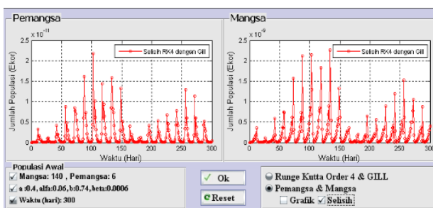
(b) Graph of the difference between RK4 and Gill estimates for predators and prey
