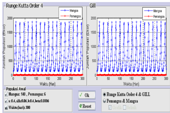
(a) Predator-Prey graph for the second case with a = b ( \alpha = 100\beta )
