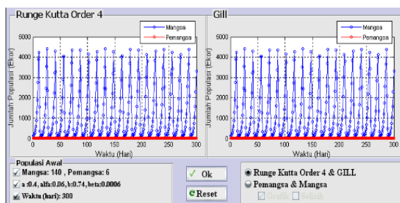
(a) Predator-Prey graph for the second case with a < b ( \alpha = 100\beta )
