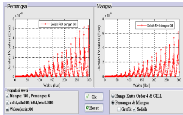
(b) Graph of the difference between RK4 and Gill estimates for predators and prey
