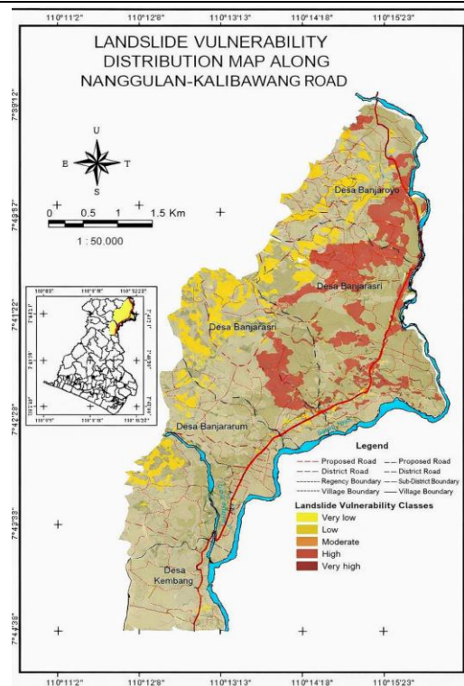
Figure 2. GIS-Based Landslide Susceptibility Map Along the Nanggulan–Kalibawang Road, Kulon Progo
