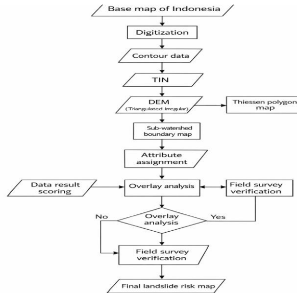
Figure 3. Scoring flowchart
