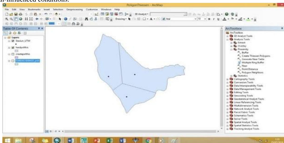
Figure 2. Poligon Thiessen overlay
